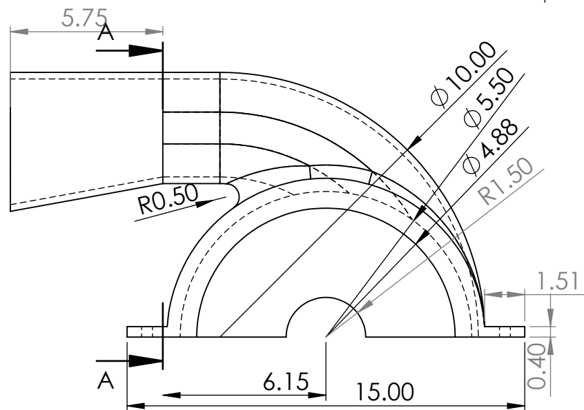
Upper Housing
