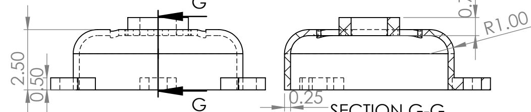
Cover
