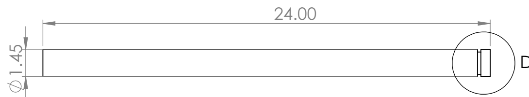
Shaft
